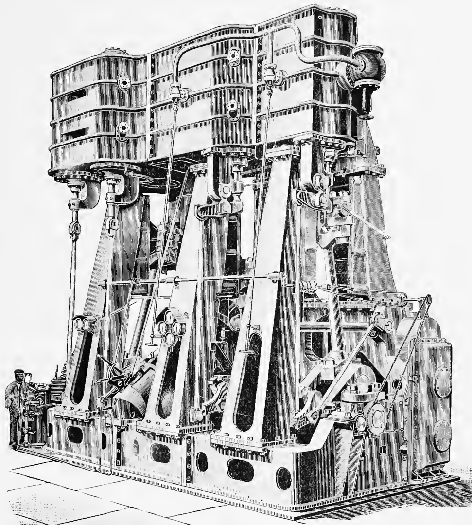
TRIPLE-EXPANSION ENGINE OF THE MORGAN LINE STEAMSHIP EL RIO.
